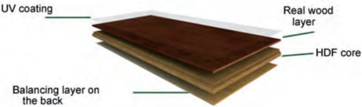
3-layers structure
