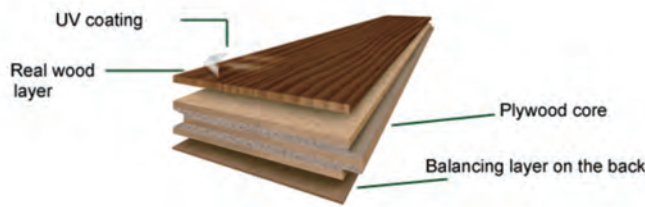
Multi-layers Structure
